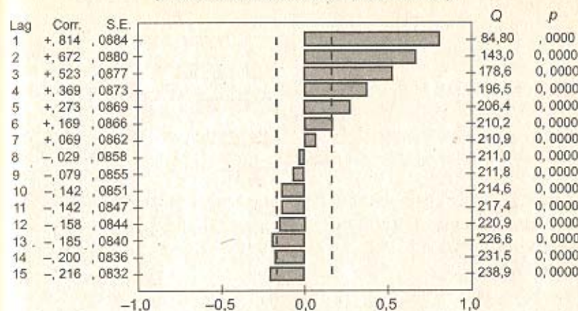
Autocorrelation Function VAR1 (Standart errors are whaite-noise estimates)
