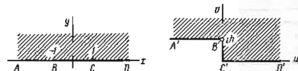
Рис. 29. w = \frac{n}{\pi} [(z^2 - 1)^{1/2} + \operatorname{Arch} z].
