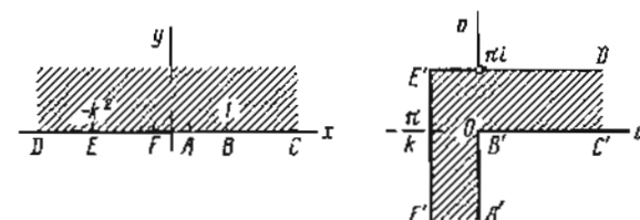
Рис. 28. w = \frac{1}{k} \ln \frac{1 + i k t}{1 - i k t} + \ln \frac{1 + i}{1 - i}; t = \left( \frac{z - 1}{z + k^2} \right)^{1/2}.
