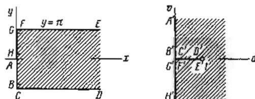
Рис. 24. w = \operatorname{cth} \frac{z}{2} = \frac{e^z + 1}{e^z - 1}.
