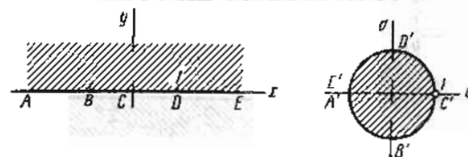
Рис. 13. w = \frac{i-z}{i+z} .
